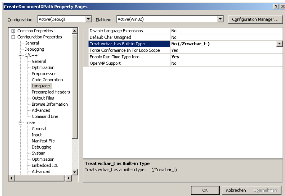
Figure 1: Changing compiler settings for using Mp7Jrs 2.x with MS VC++ .NET 2005.
